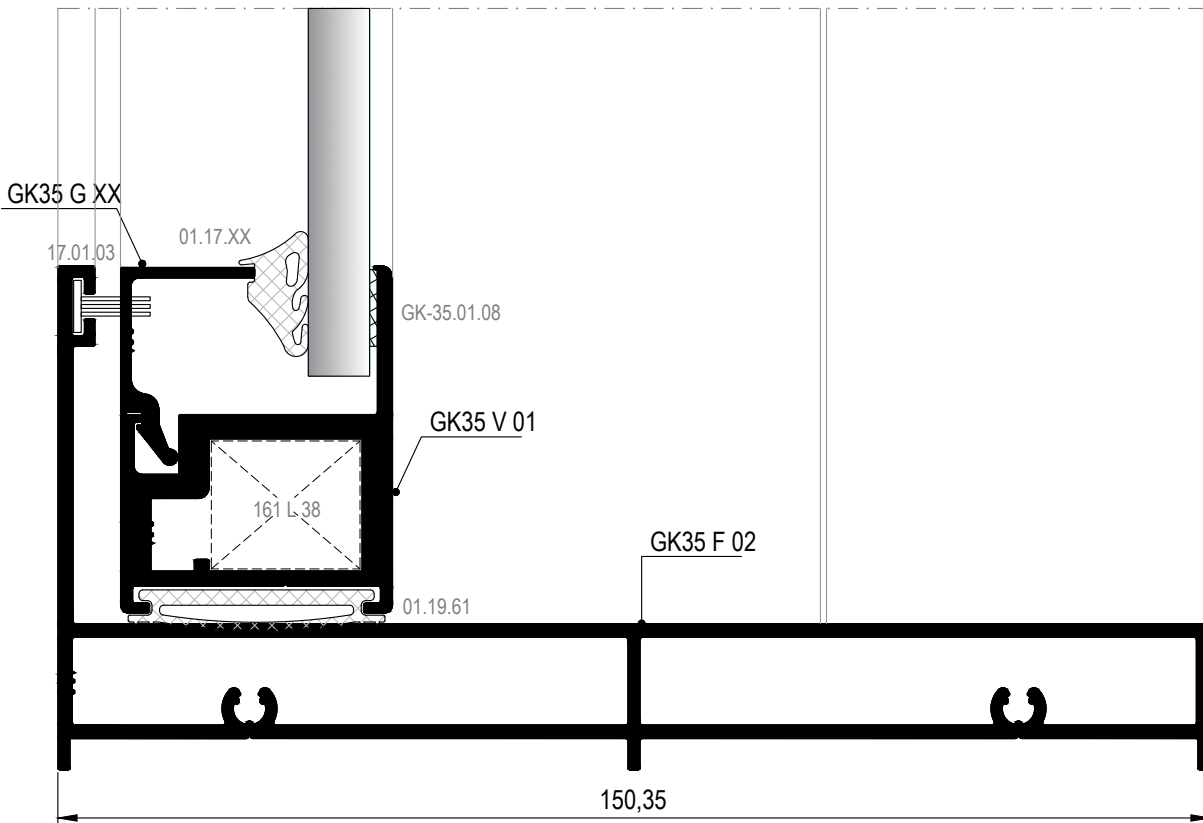
18 DETAYI DETAIL
