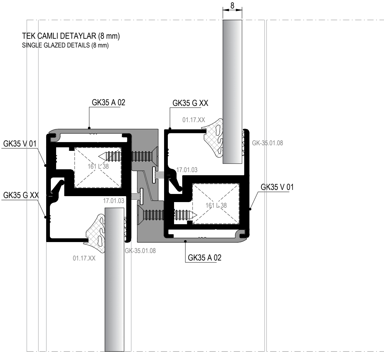
17 DETAYI DETAIL
