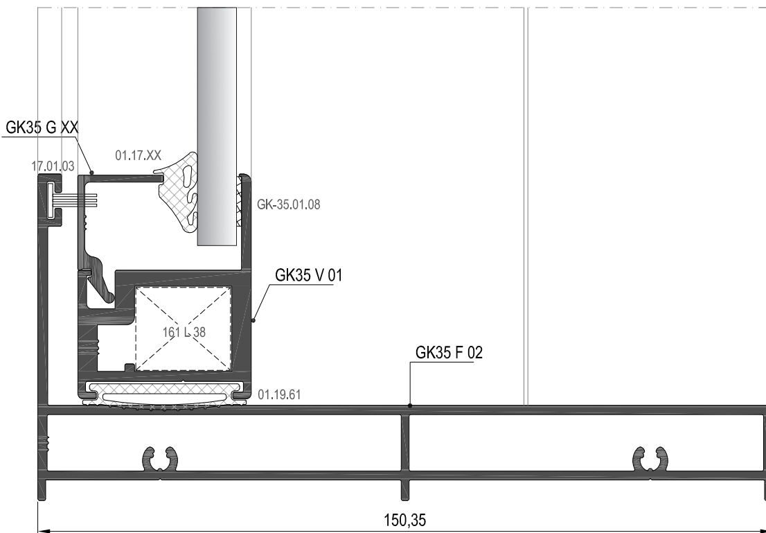
18 DETAYI DETAIL
