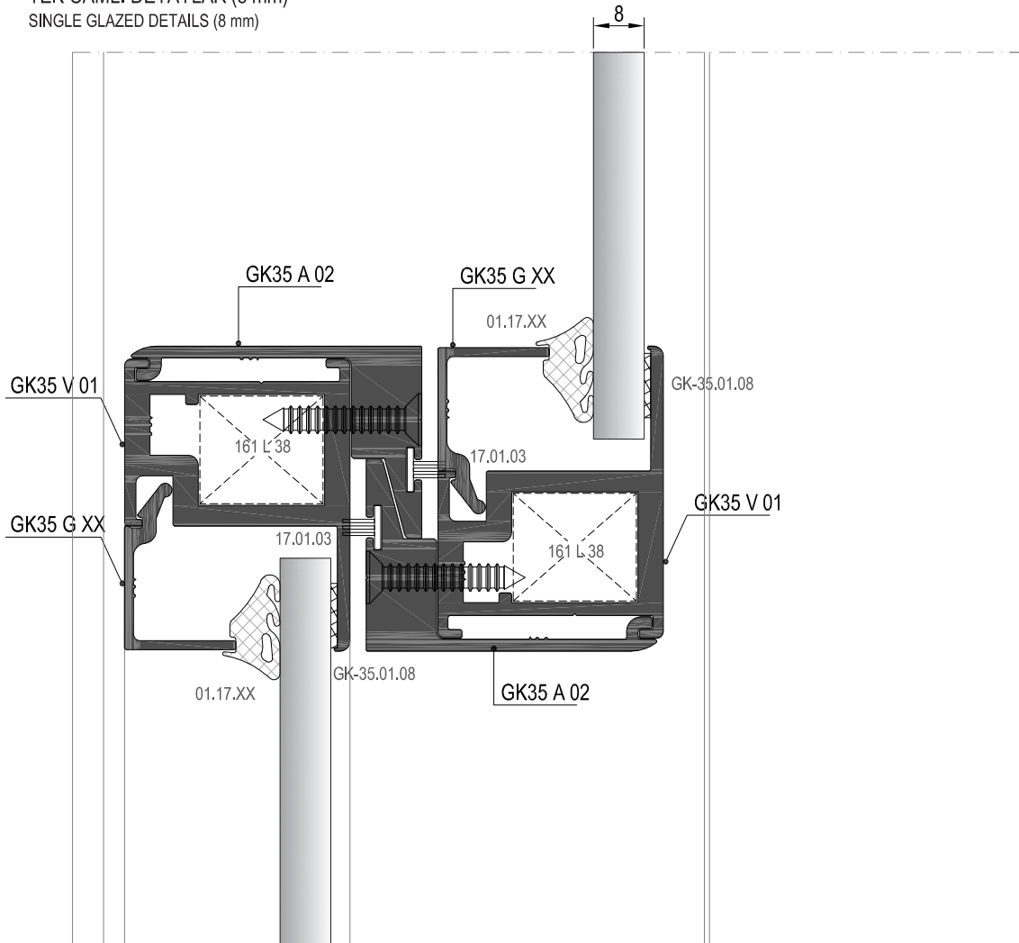
17 DETAYI DETAIL
